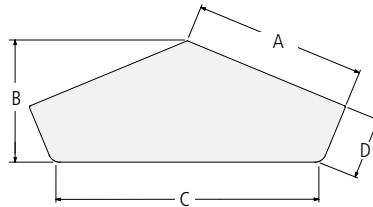
135-Degree Bridge Dimensions
