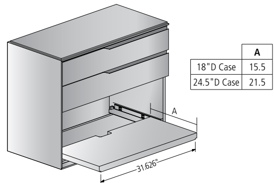
Pull-Out Equipment Tray
