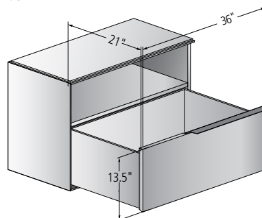
Center Box / Large Box Drawer OS1LD
