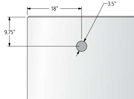
Thermostatically-Controlled Fan Cutout in Back Panel
