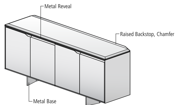
Buffet Height with Metal Base Beveled Case
