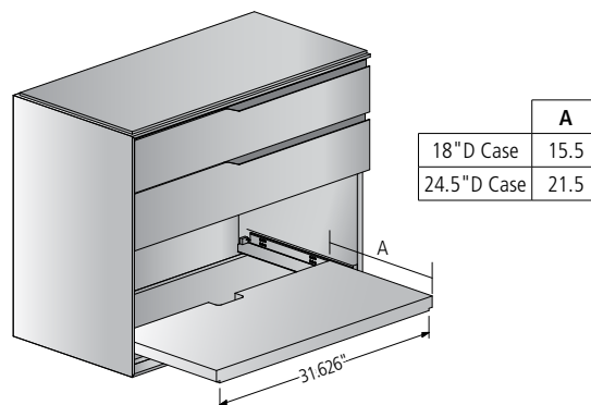
Pull-Out Equipment Tray
