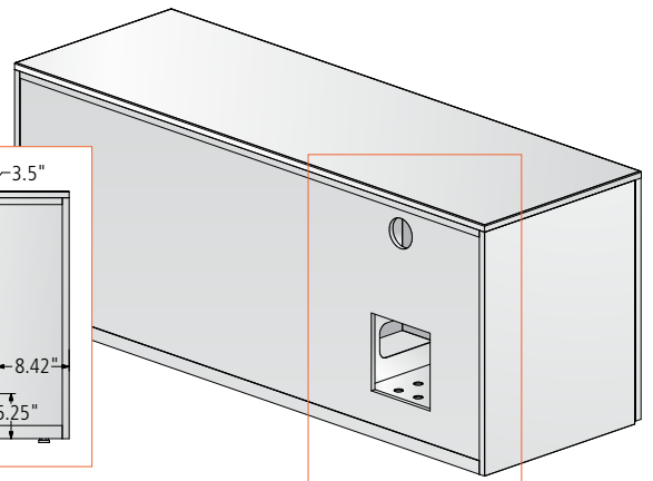
Racked Equipment Cutout
