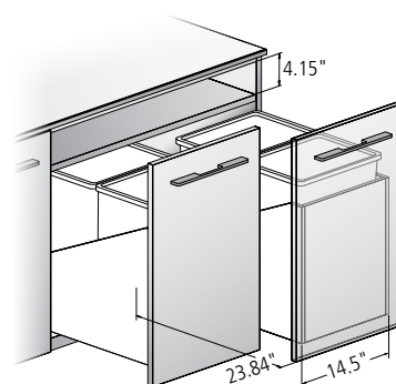
Dual Wood Frame Double Waste/Recycling Unit
