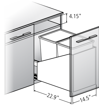
Wood Frame Double Waste/Recycling Unit
