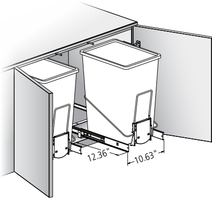
Dual Wire Frame Single Waste/Recycling Unit
