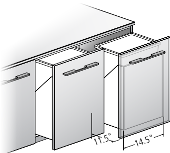
Dual Wood Frame Single Waste/Recycling Unit
