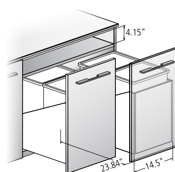
Dual Wood Frame Double Waste/Recycling Unit
