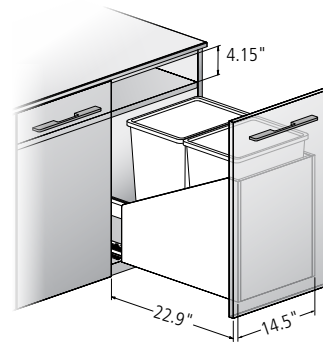
Dual Wire Frame Double Waste/Recycling Unit
