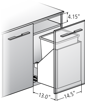
Wood Frame Single Waste/Recycling Unit
