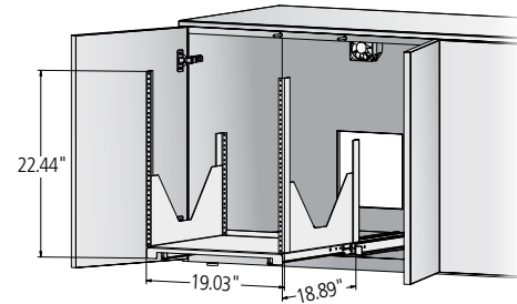
Sliding Equipment Rack
