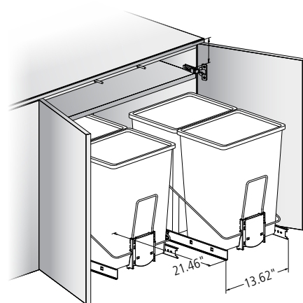
Dual Wood Frame Double Waste/Recycling Unit
