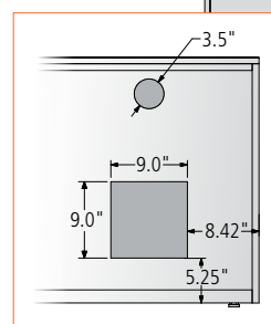
Racked Equipment Cutout
