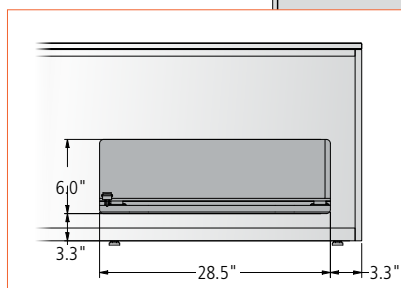
Drawer Refrigerator Cutout
