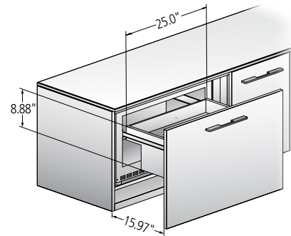
Pull-out Drawer Refrigerator
