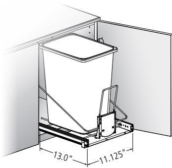
Wire Frame Single Waste/Recycling Unit
