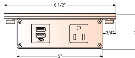
Power Block (Simplex / Charging USB)
