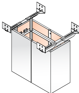
Four Post Base, T-Base and Hoop Base (Structural Support Center Column)
