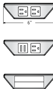
Front Elevation
