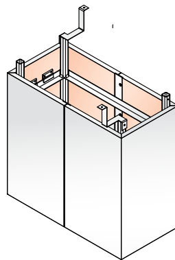
Four Post Base, T-Base and Hoop Base (Non-Structural Support Center Column)
