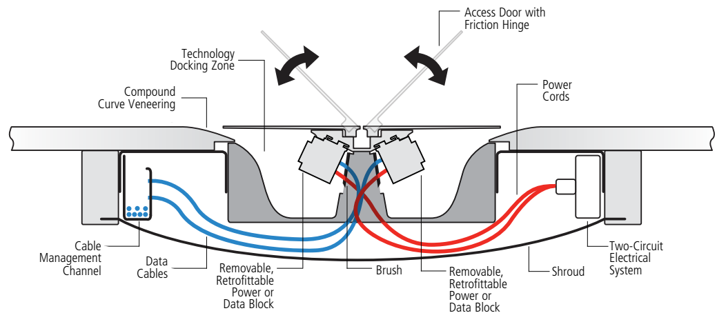
Front Elevation
