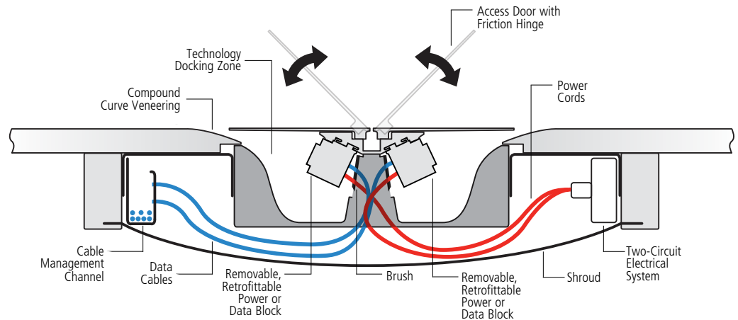
Front Elevation
