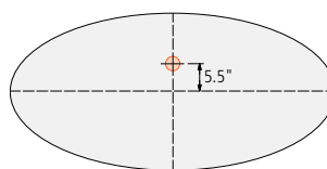
PD-36 Ellipse Power Dot Location
