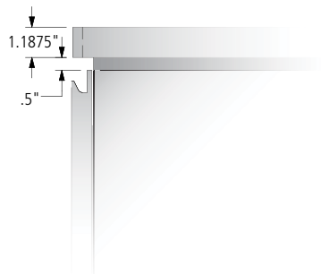
Veneer with Square (SQ) Edge
