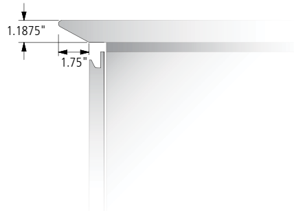
Veneer with Radius Knife (RK) Edge
