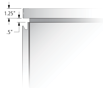
Laminate with Square Edge
