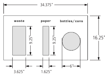
3 Station Unit
