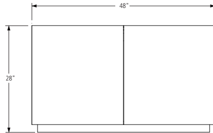
4 Station Unit
