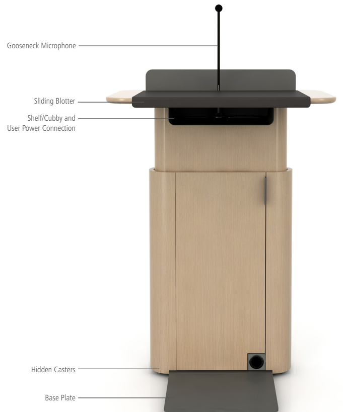
Height Adjustable Lectern
