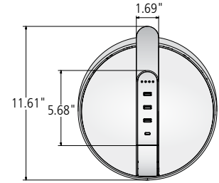
Battery-Powered Charging Stand Top View
