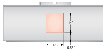
72" - Back Panel Cutout
