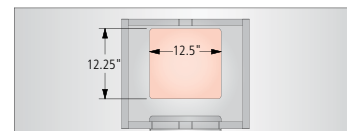
60" - Top Panel Cutout
