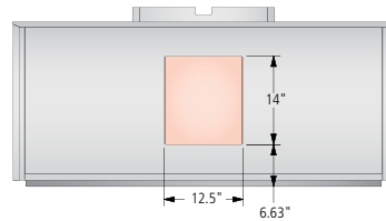
60" - Back Panel Cutout
