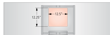
72" - Top Panel Cutout
