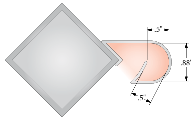
Top View Post Leg with Wire Management Channel
